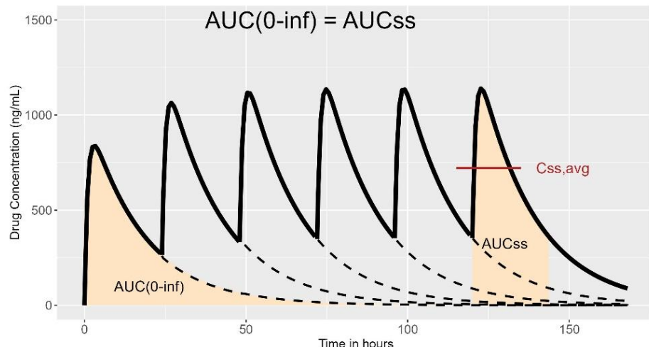
Figure 33. Concentration-time profile after multiple doses of a drug given once daily. For a drug having linear pharmacokinetics, the AUC of the concentration-time profile from time 0 to infinity (shown as the beige band) is equal to the AUC under the dosing interval at steady-state ( AUC_{ss} , shown in the beige band after the 6 th dose). For this simulation, a dose of 100 mg was given once daily. The volume of distribution of the drug was 100 L, the absorption rate constant was 1 per h, and the half-life was 12 h. The average steady-state concentration ( C_{ss,avg} ) is represented by the red line.
