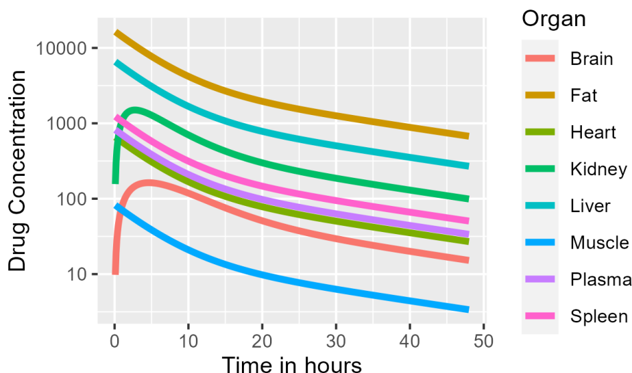
Figure 27: Drug concentration-time profiles in various organs after single-dose intravenous administration.
